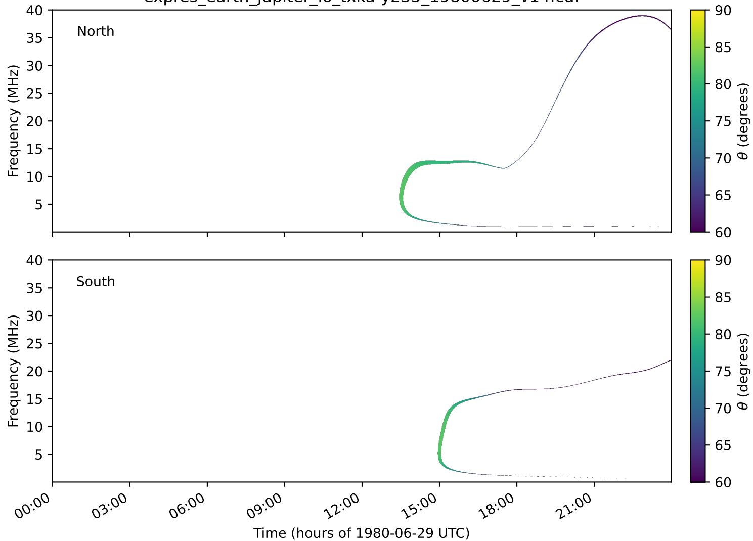
expres_earth_jupiter_io_txka-y235_19800629_v14.cdf
