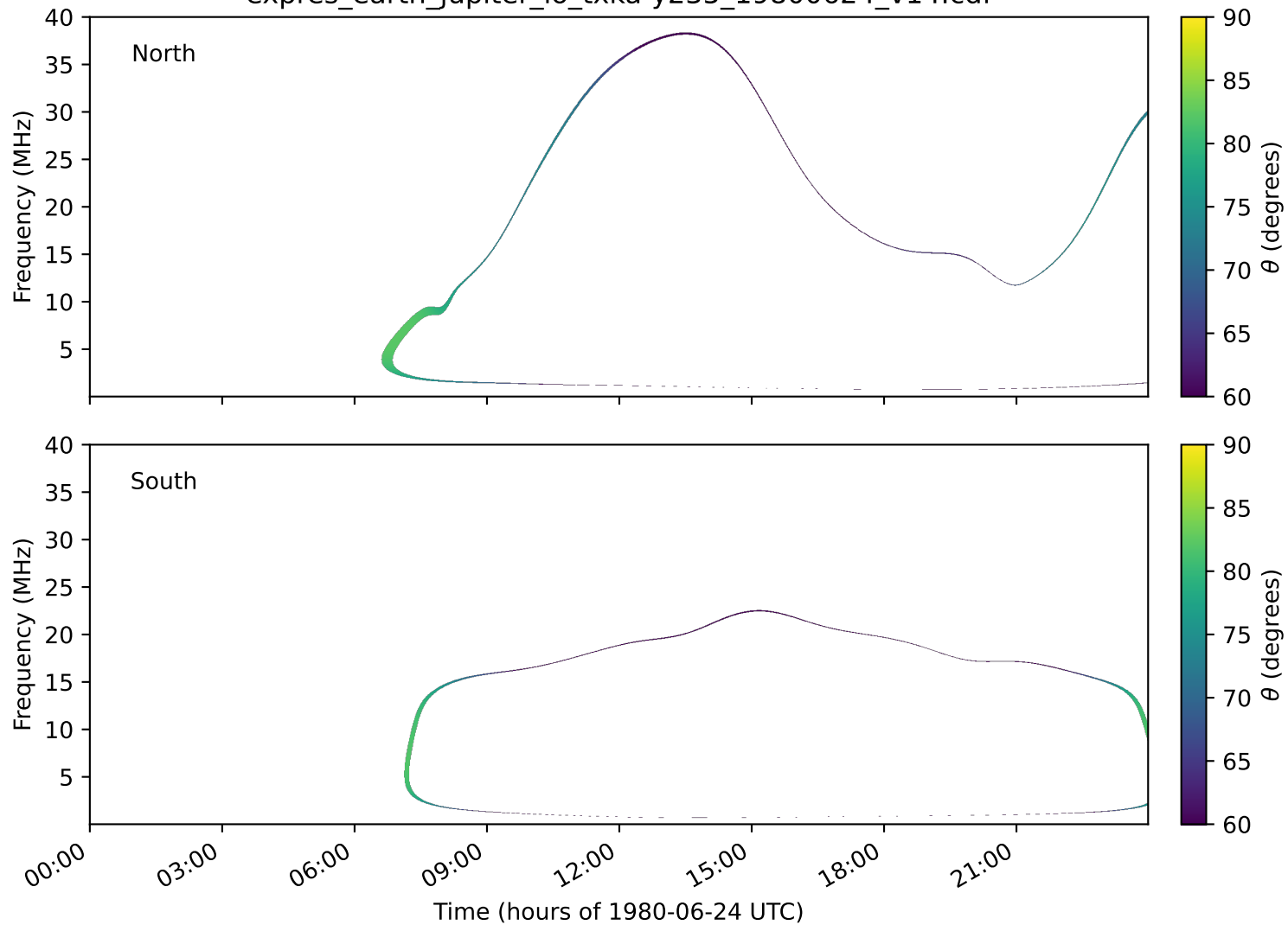
expres_earth_jupiter_io_txka-y235_19800624_v14.cdf
