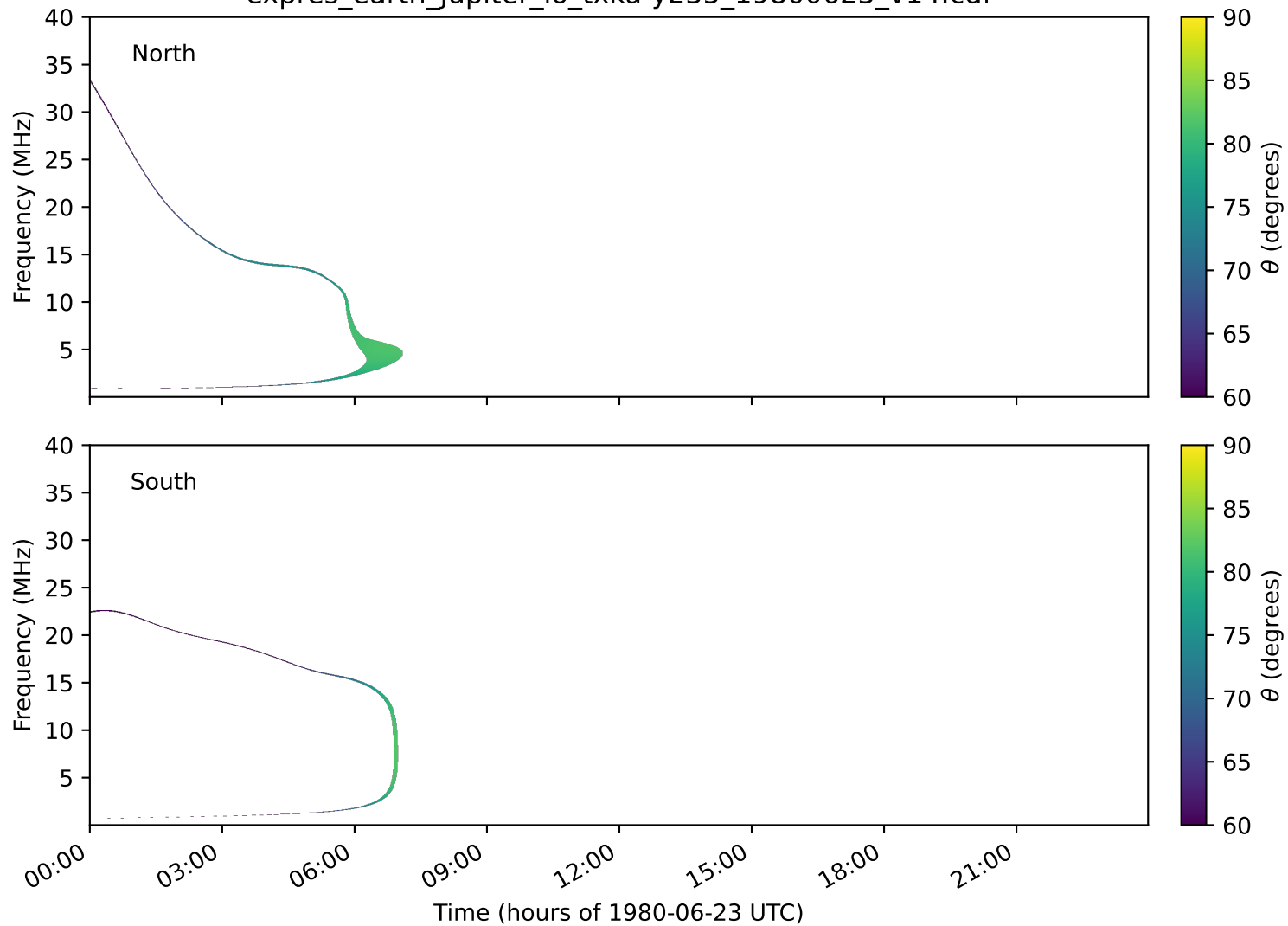
expres_earth_jupiter_io_txka-y235_19800623_v14.cdf
