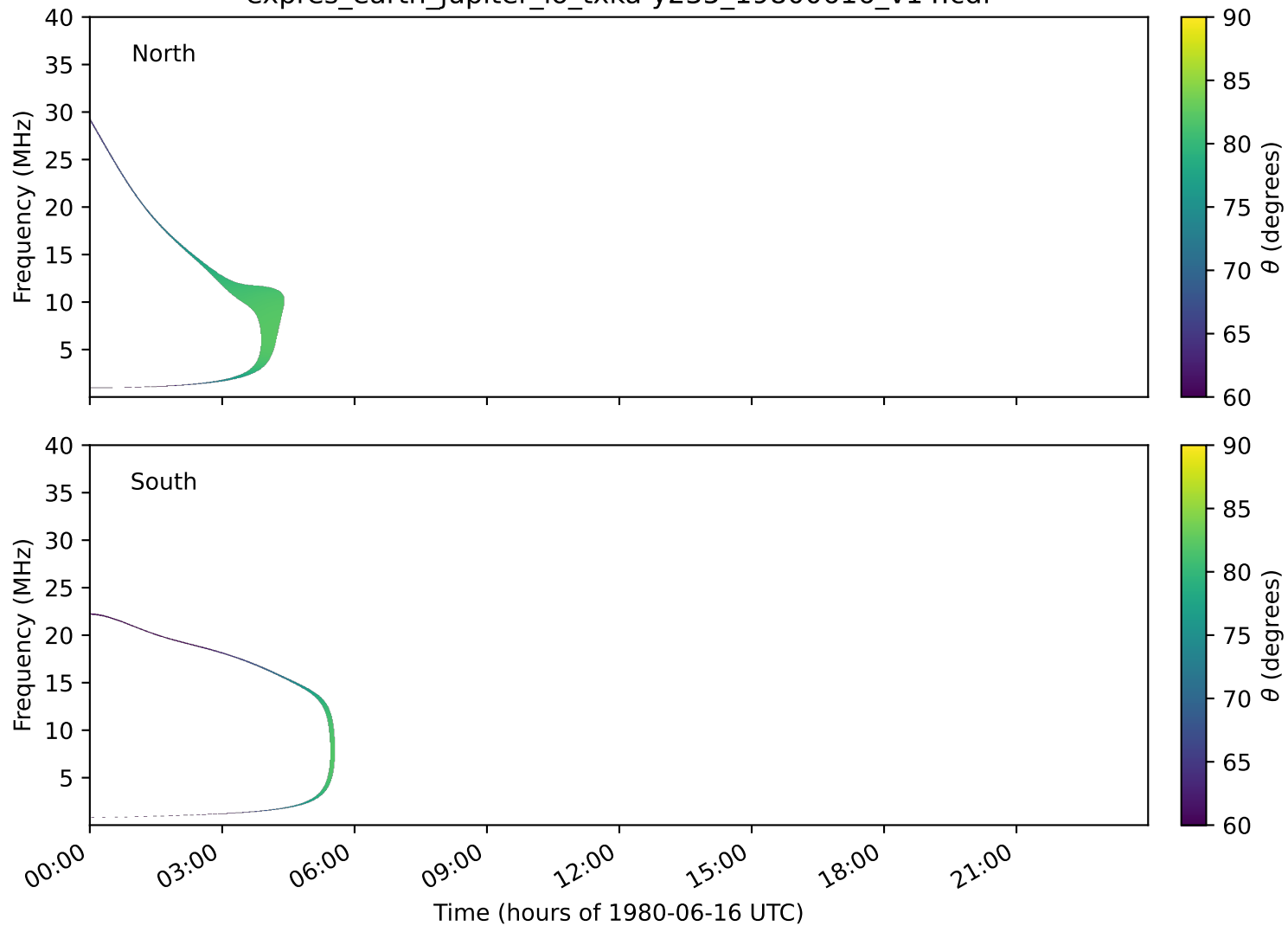
expres_earth_jupiter_io_txka-y235_19800616_v14.cdf
