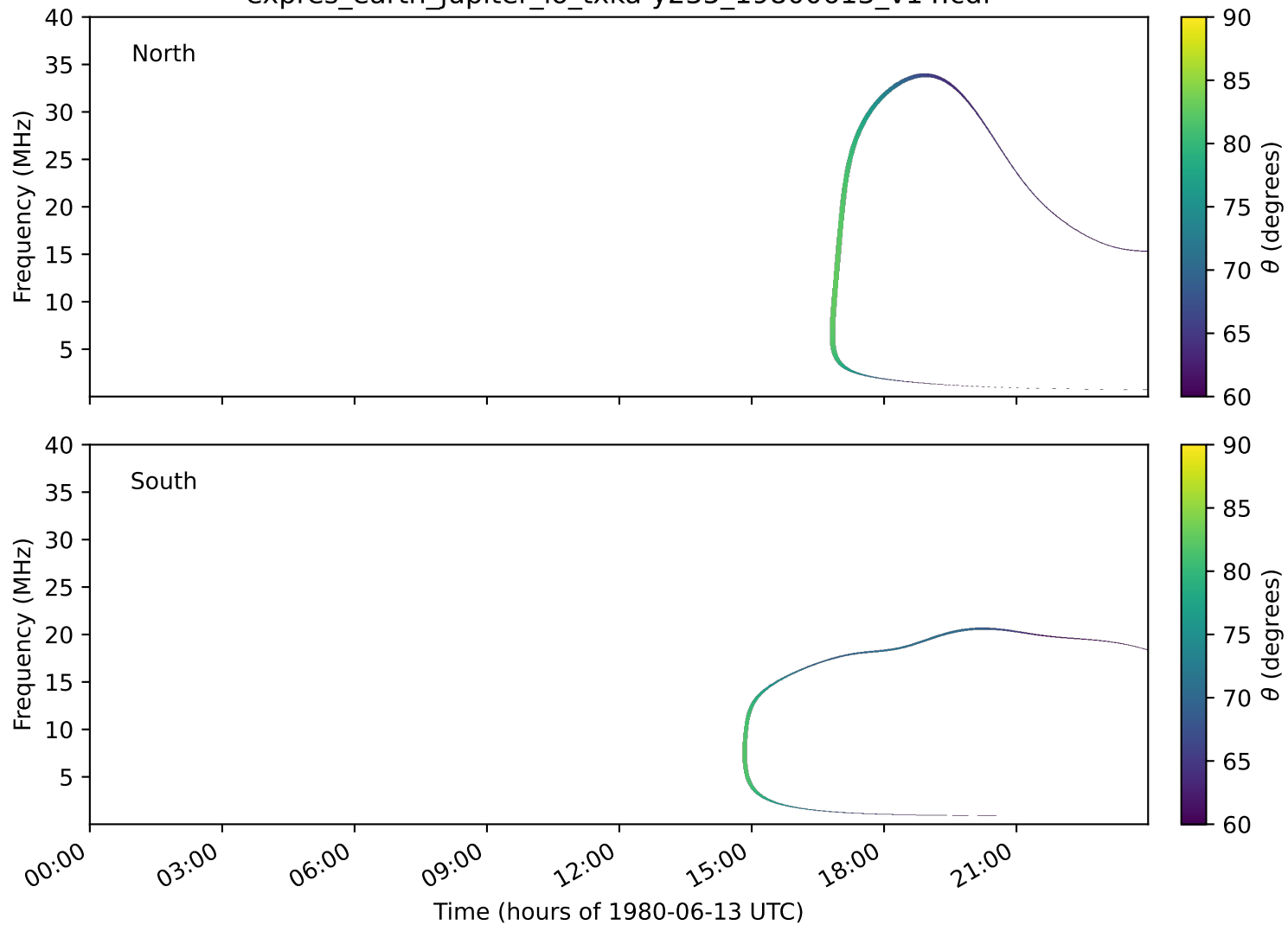
expres_earth_jupiter_io_txka-y235_19800613_v14.cdf
