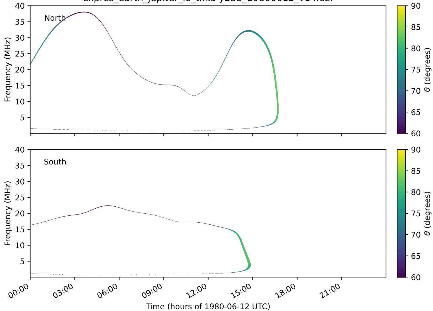
expres_earth_jupiter_io_txka-y235_19800612_v14.cdf
