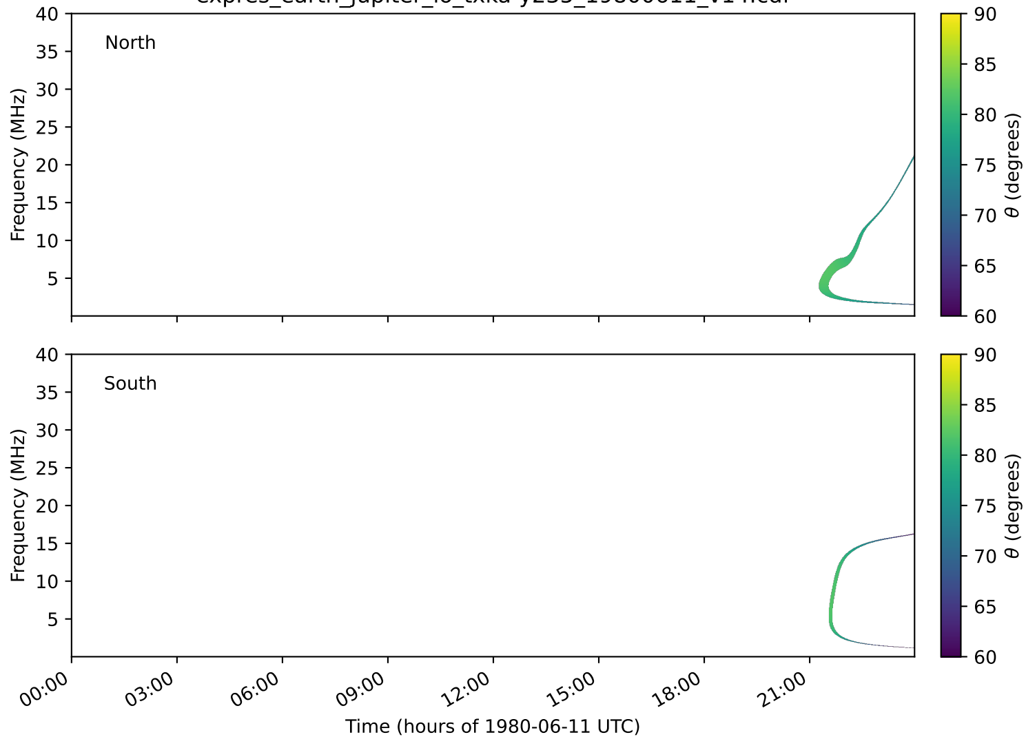
expres_earth_jupiter_io_txka-y235_19800611_v14.cdf
