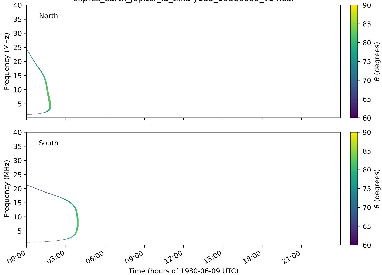
expres_earth_jupiter_io_txka-y235_19800609_v14.cdf
