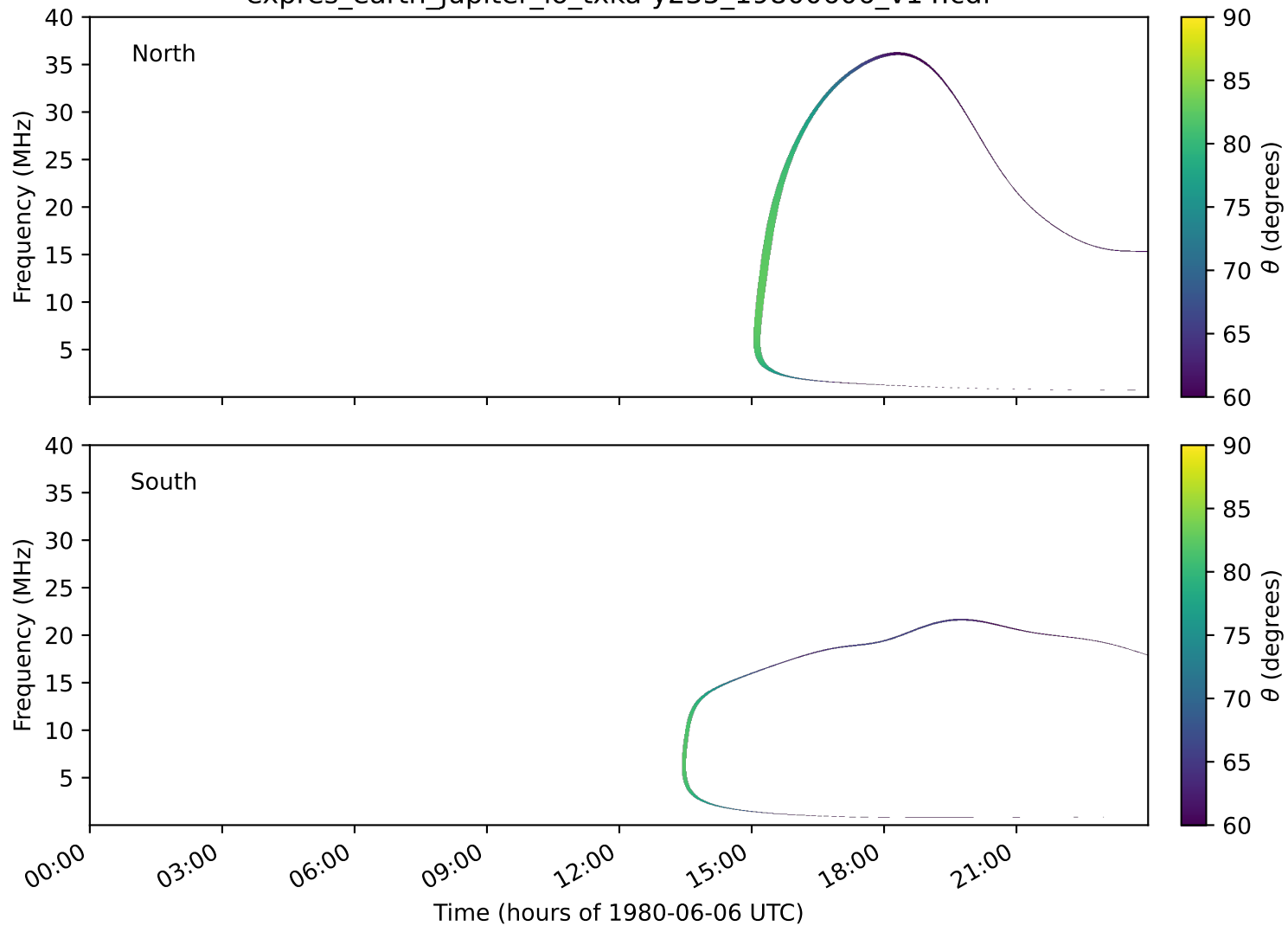
expres_earth_jupiter_io_txka-y235_19800606_v14.cdf
