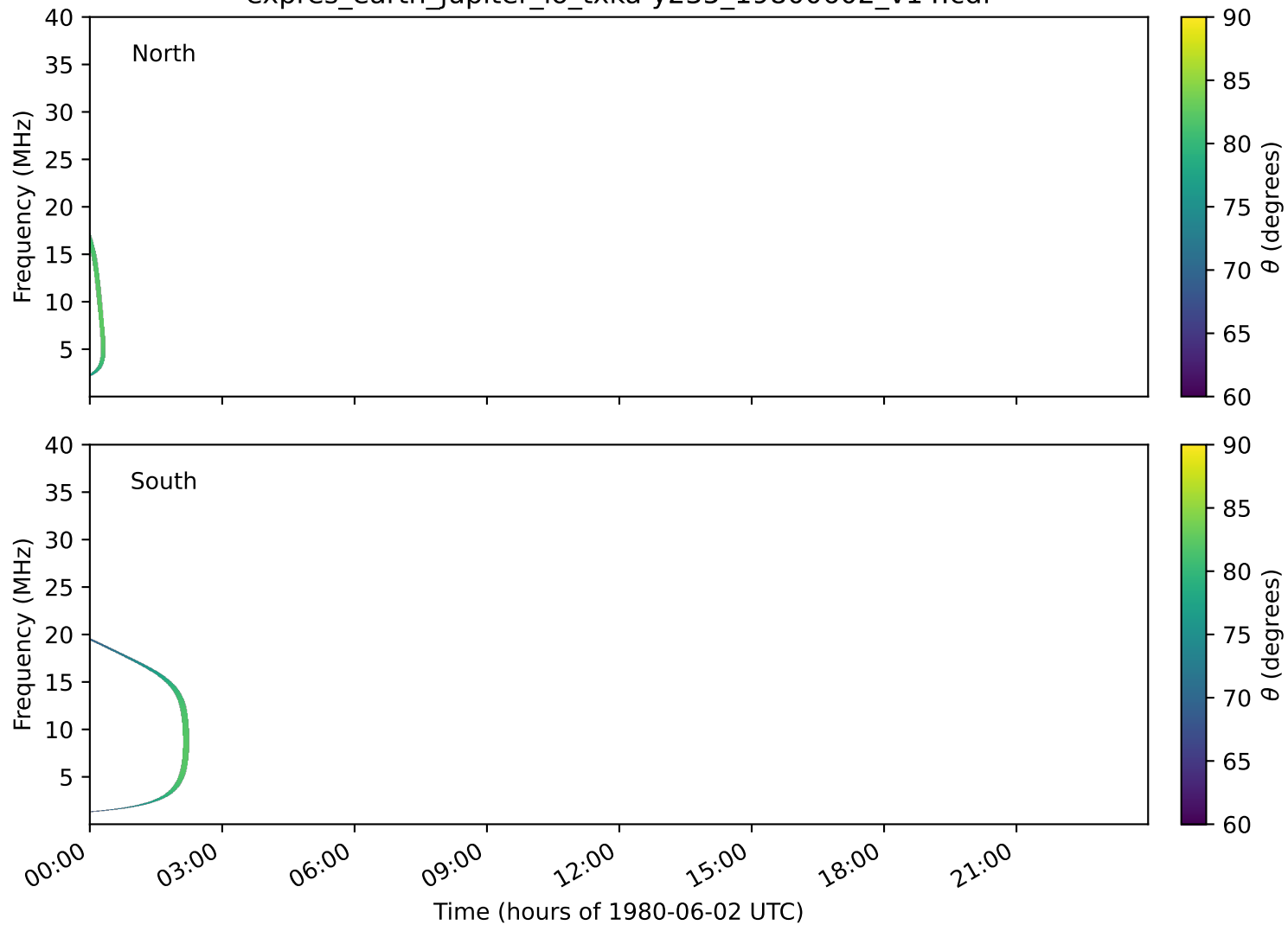
expres_earth_jupiter_io_txka-y235_19800602_v14.cdf
