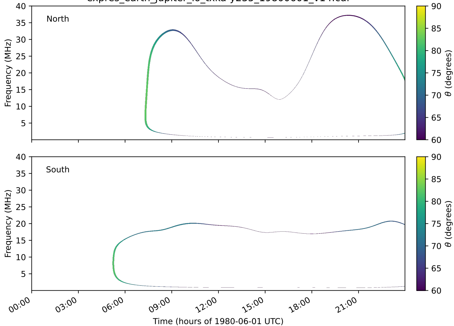
expres_earth_jupiter_io_txka-y235_19800601_v14.cdf
