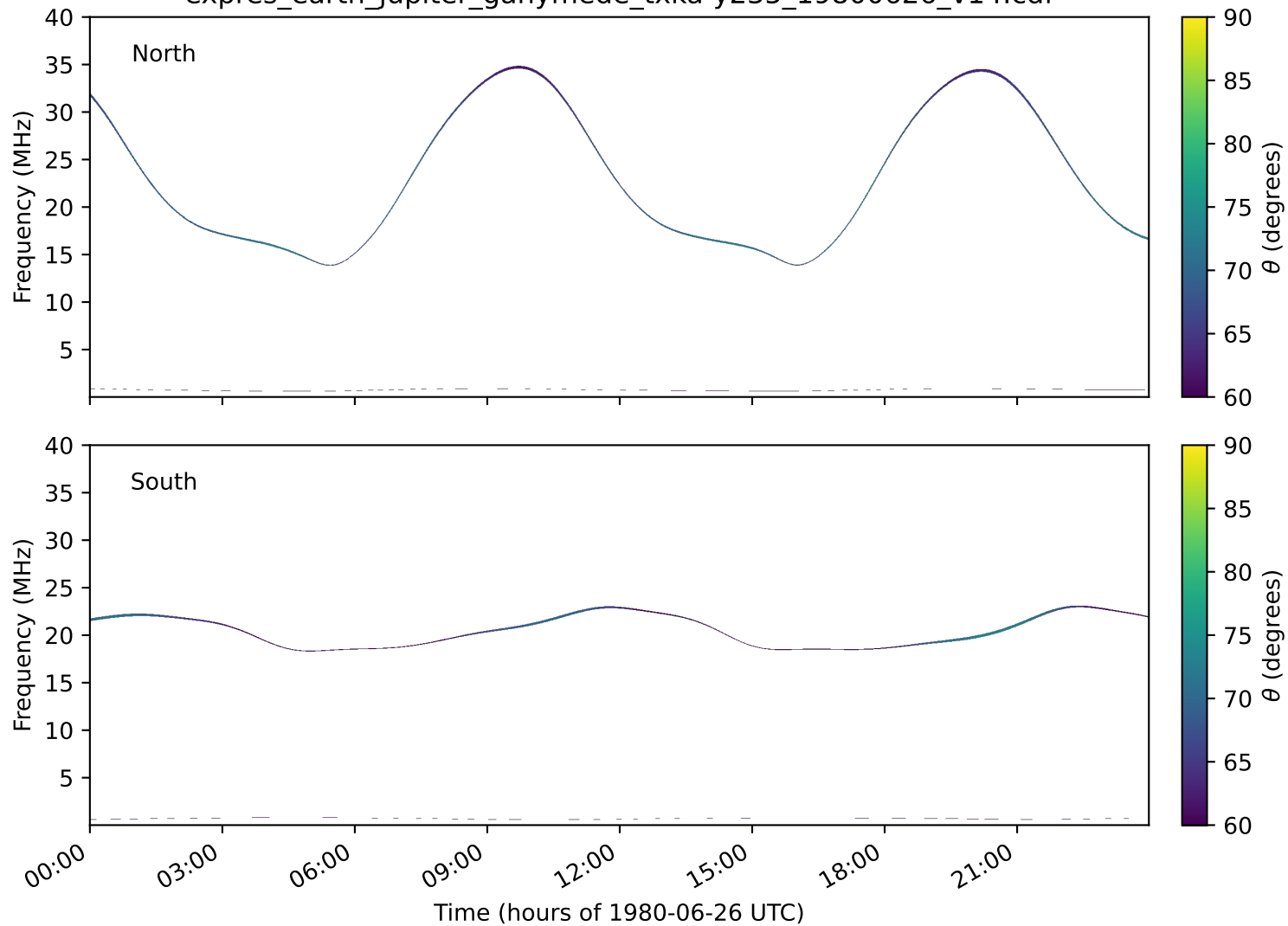
expres_earth_jupiter_ganymede_txka-y235_19800626_v14.cdf
