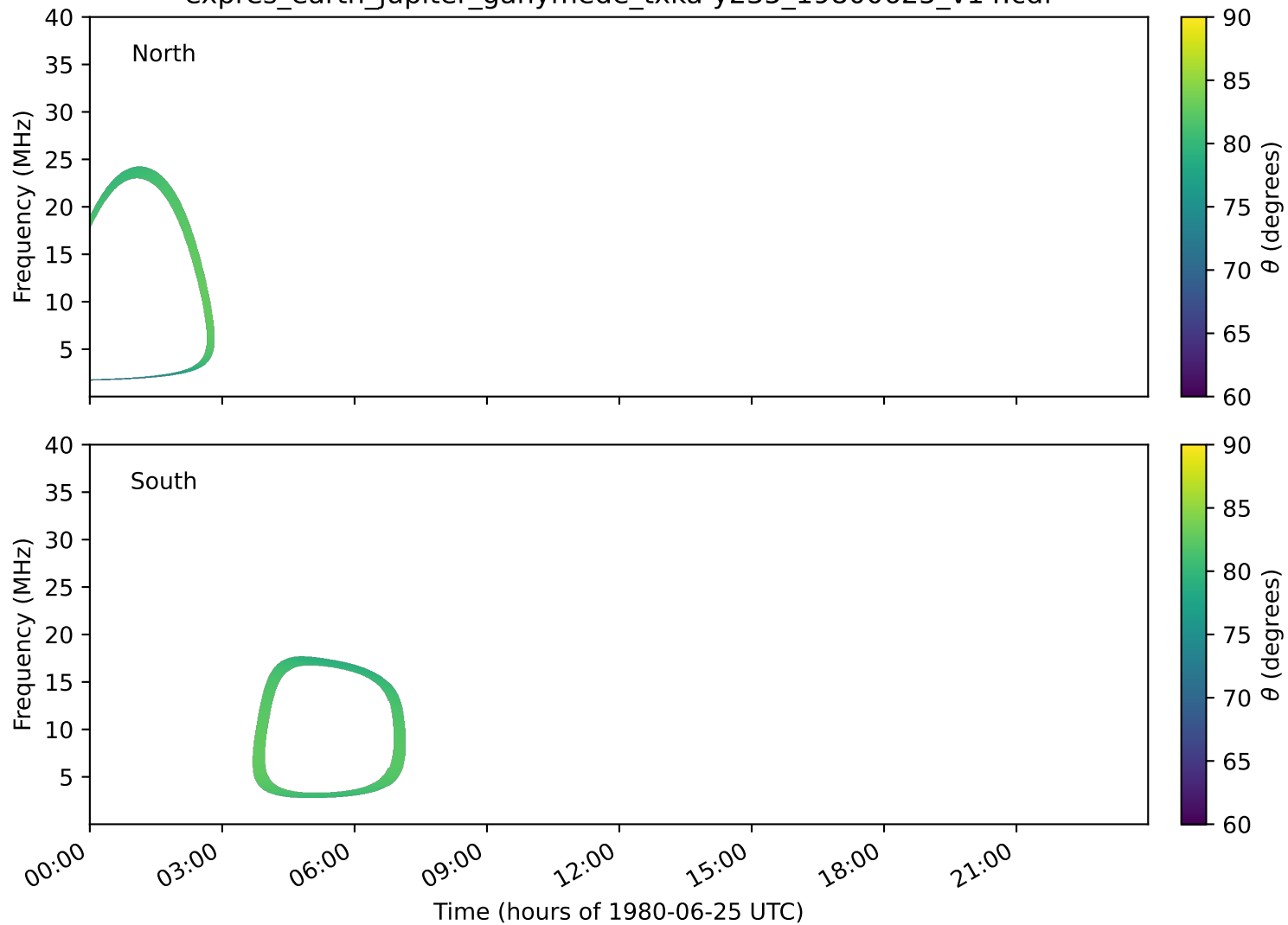
expres_earth_jupiter_ganymede_txka-y235_19800625_v14.cdf
