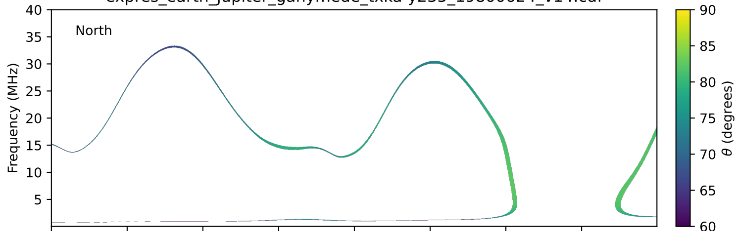
expres_earth_jupiter_ganymede_txka-y235_19800624_v14.cdf
