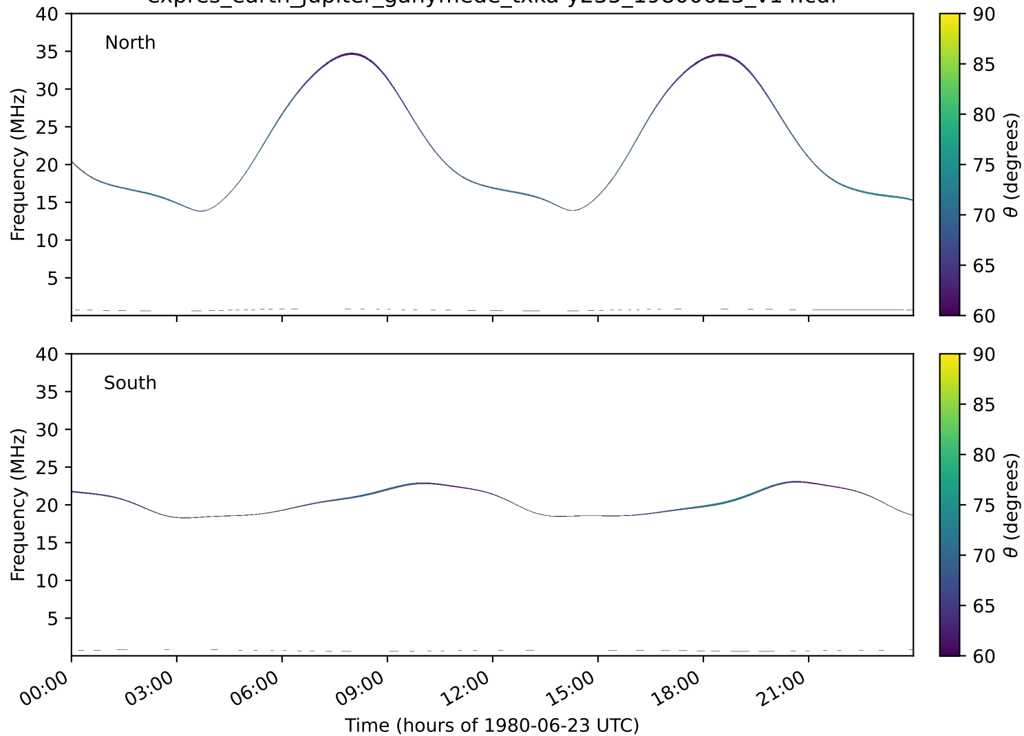
expres_earth_jupiter_ganymede_txka-y235_19800623_v14.cdf
