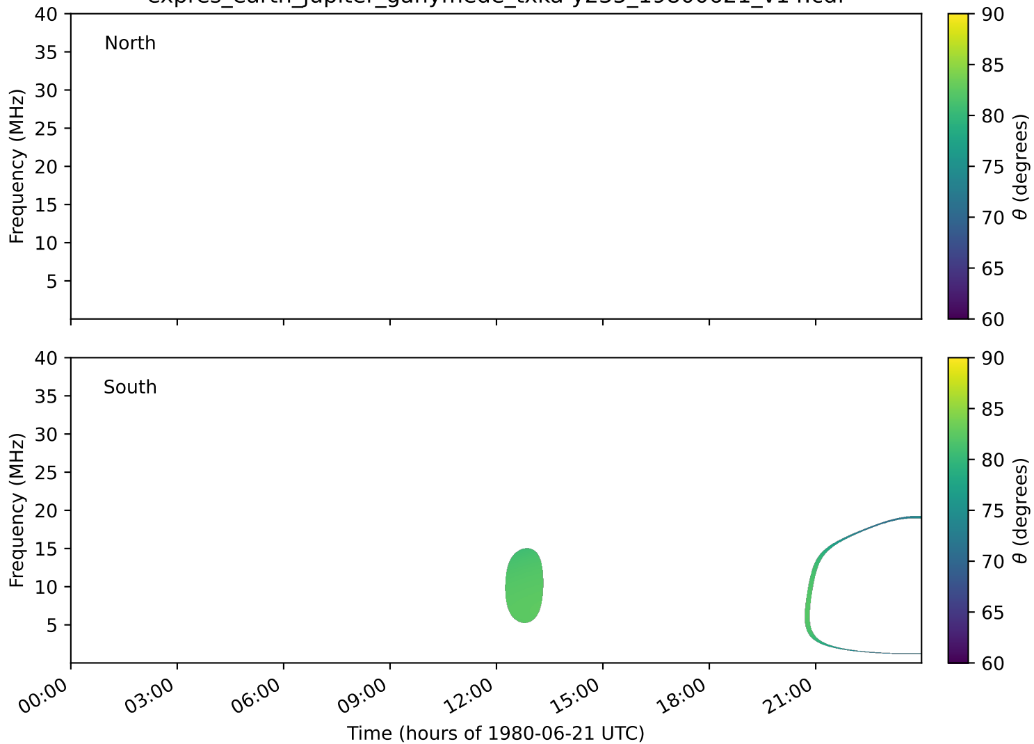
expres_earth_jupiter_ganymede_txka-y235_19800621_v14.cdf
