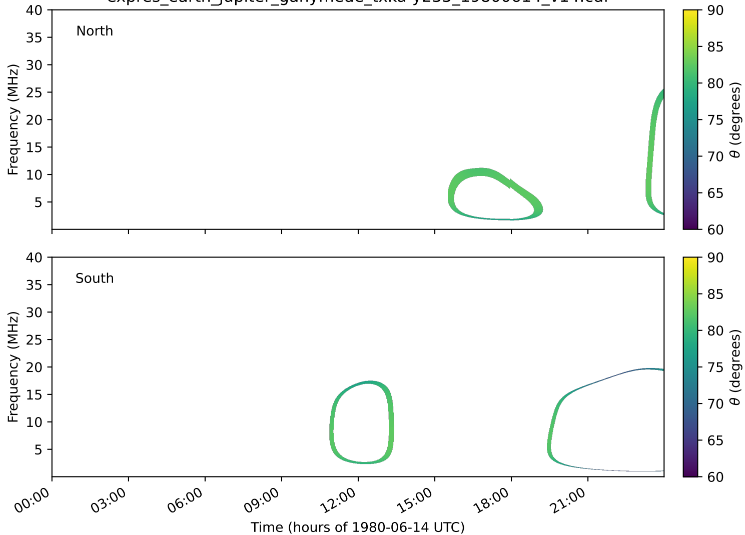
expres_earth_jupiter_ganymede_txka-y235_19800614_v14.cdf
