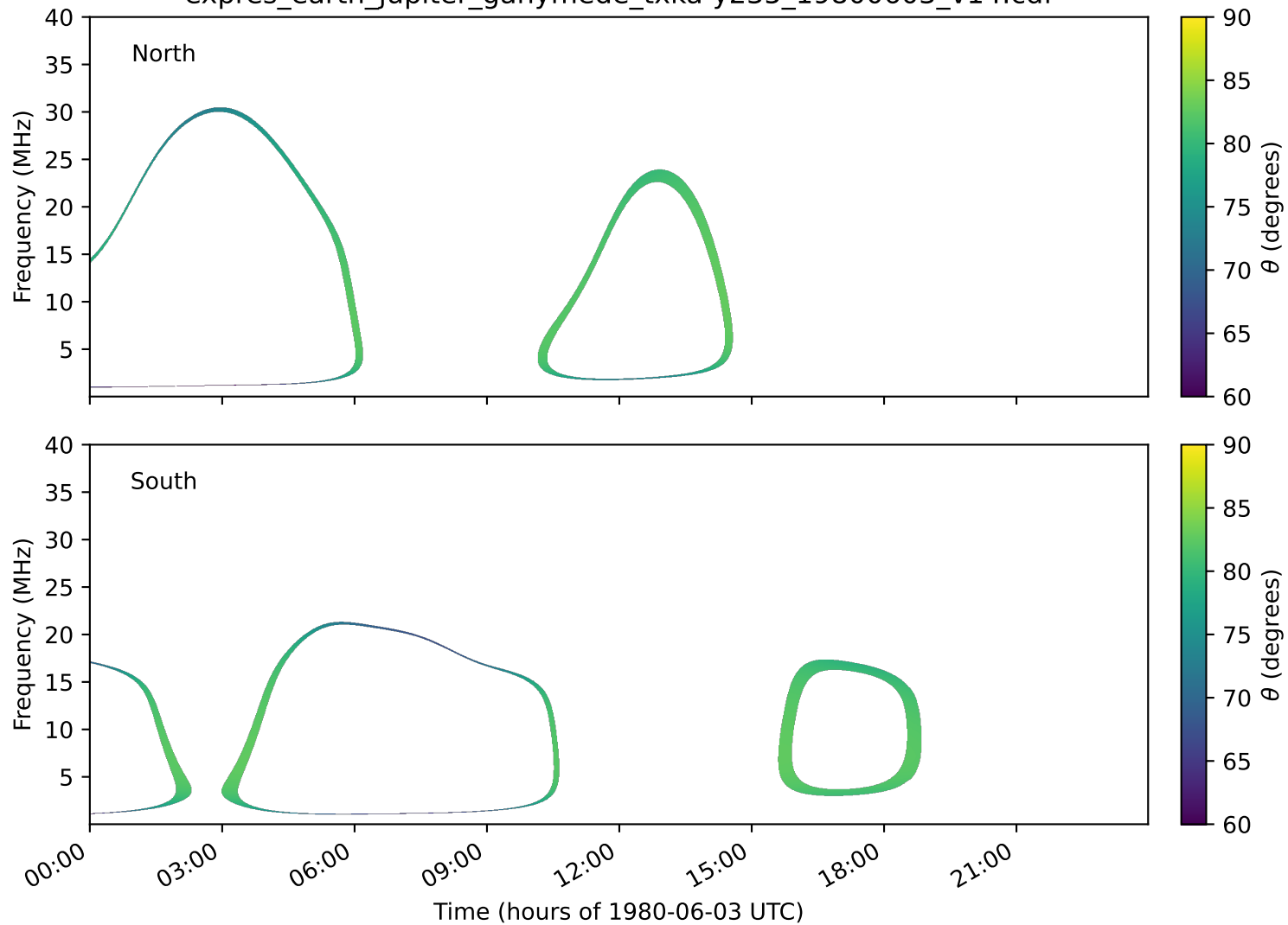
expres_earth_jupiter_ganymede_txka-y235_19800603_v14.cdf
