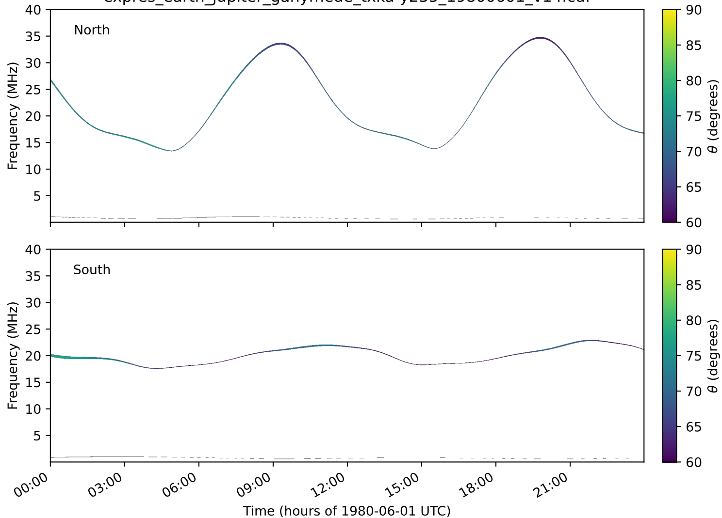
expres_earth_jupiter_ganymede_txka-y235_19800601_v14.cdf
