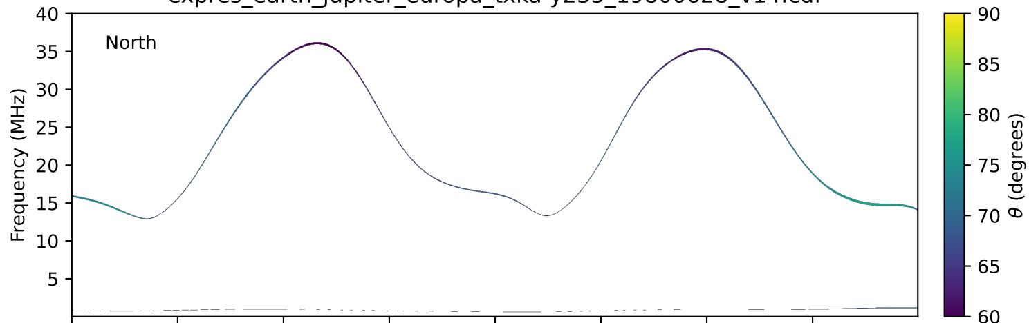
expres_earth_jupiter_europa_txka-y235_19800628_v14.cdf
