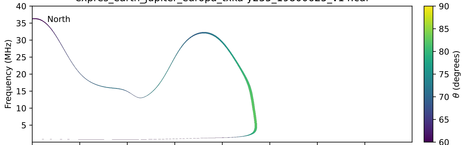
expres_earth_jupiter_europa_txka-y235_19800625_v14.cdf
