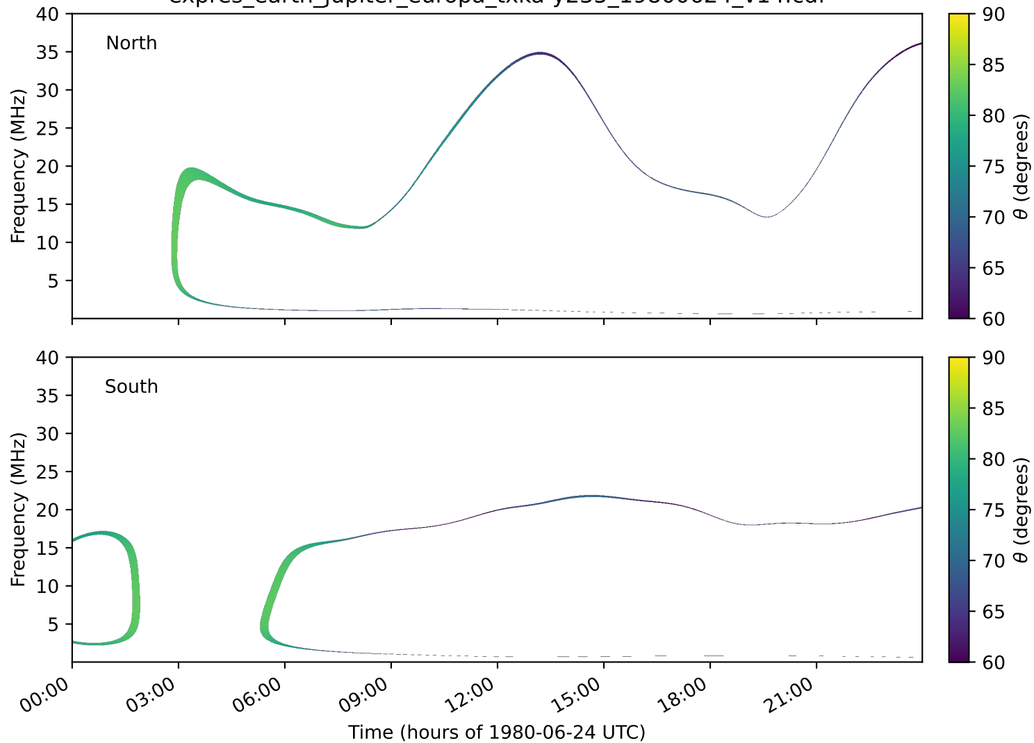
expres_earth_jupiter_europa_txka-y235_19800624_v14.cdf
