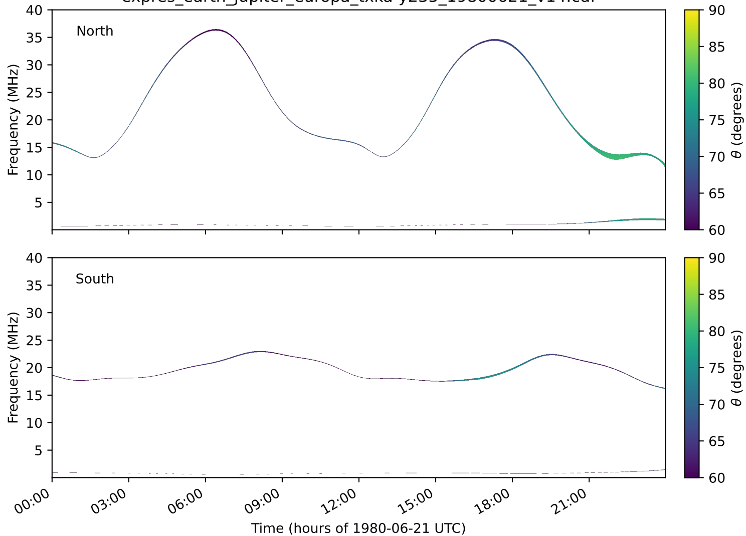
expres_earth_jupiter_europa_txka-y235_19800621_v14.cdf
