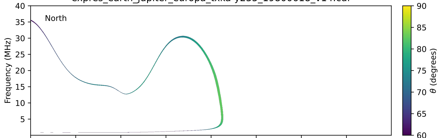
expres_earth_jupiter_europa_txka-y235_19800618_v14.cdf
