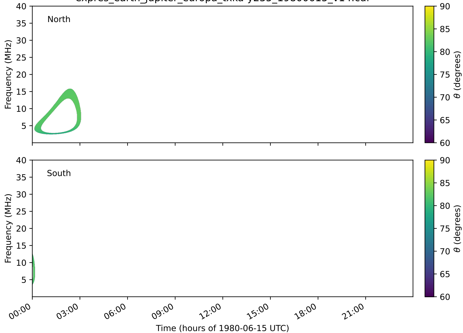
expres_earth_jupiter_europa_txka-y235_19800615_v14.cdf
