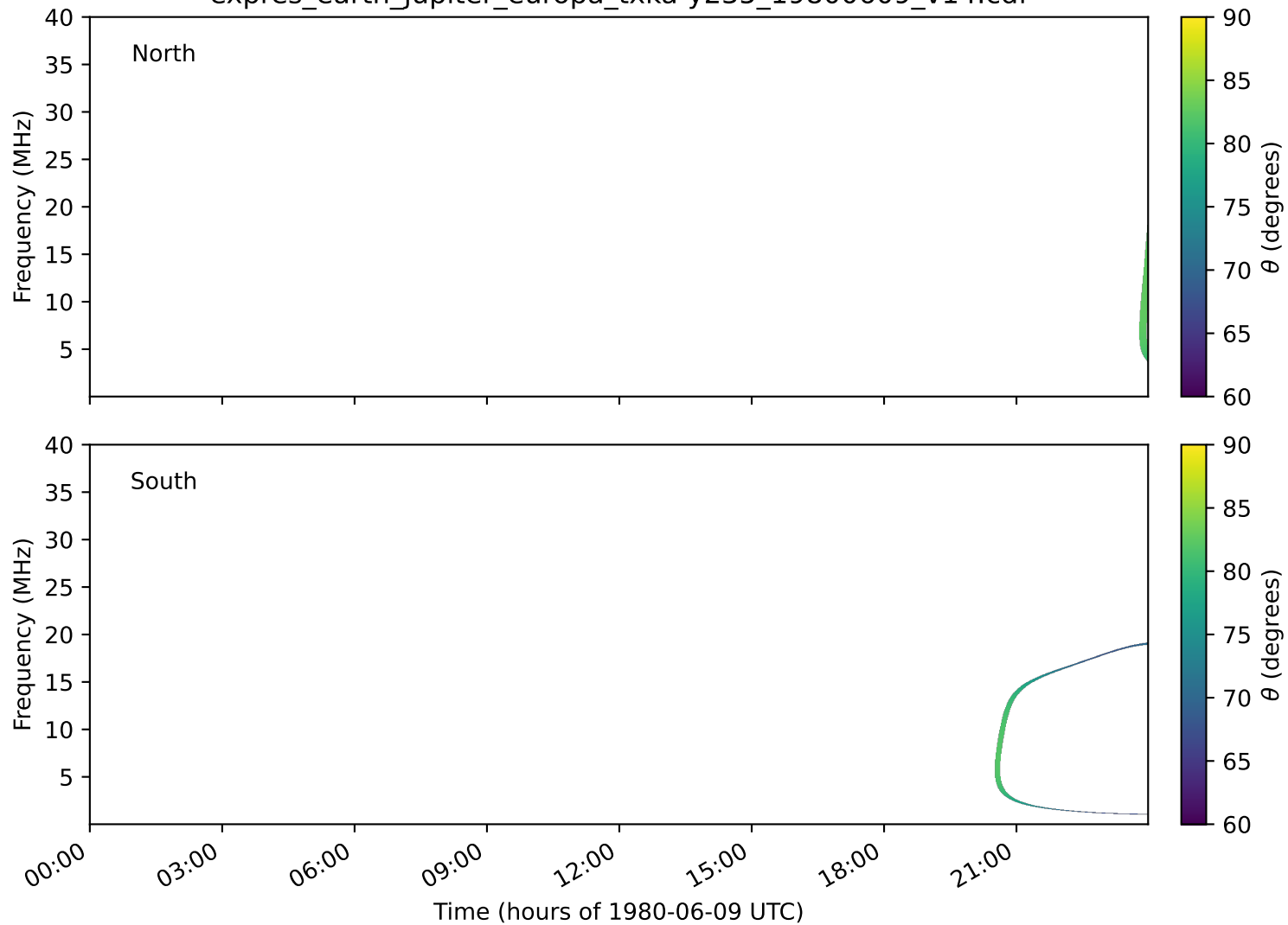
expres_earth_jupiter_europa_txka-y235_19800609_v14.cdf
