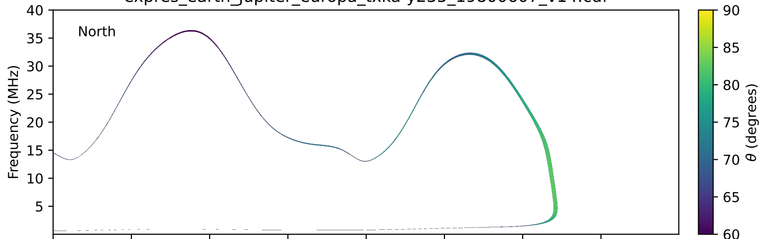
expres_earth_jupiter_europa_txka-y235_19800607_v14.cdf
