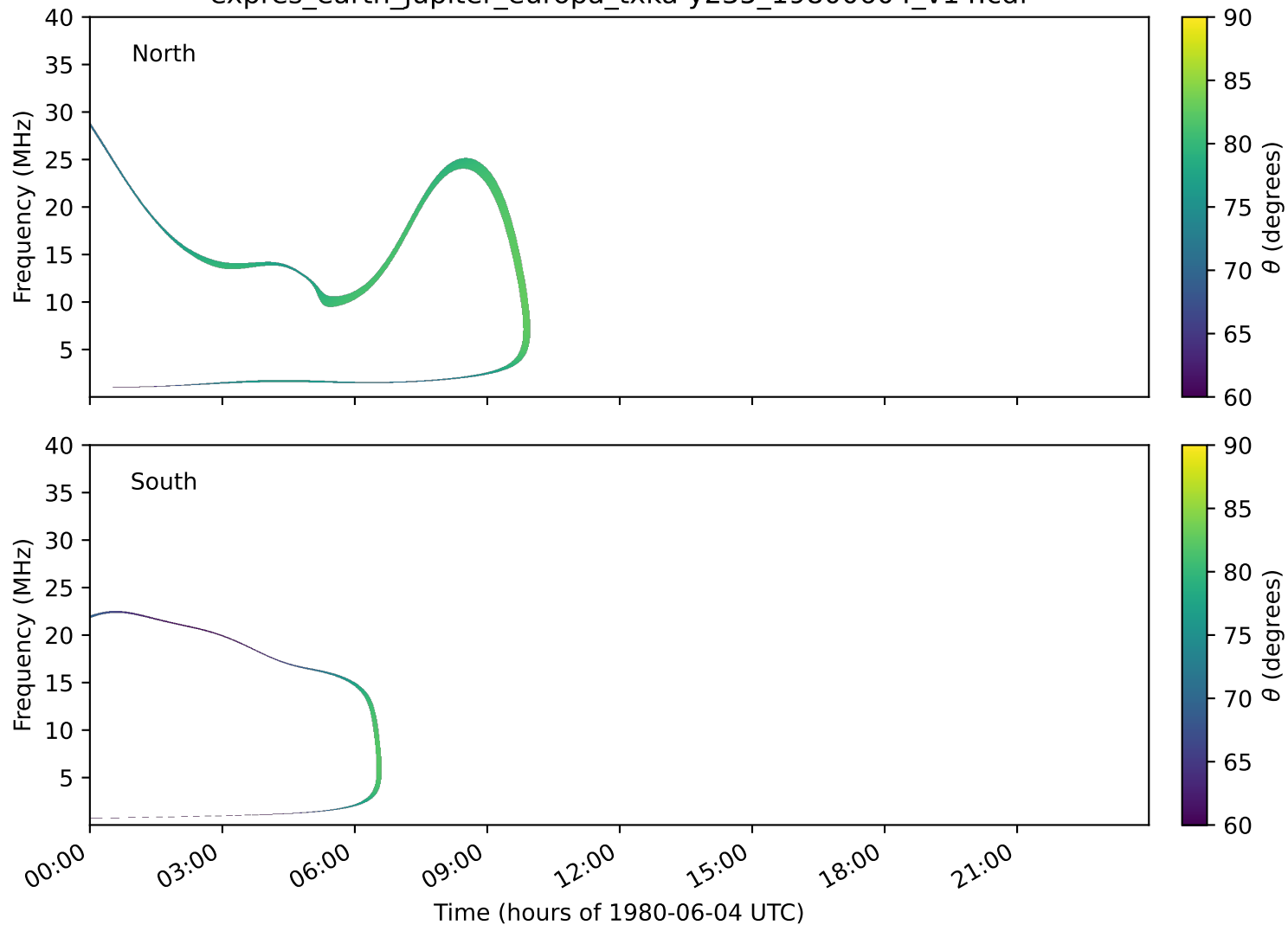
expres_earth_jupiter_europa_txka-y235_19800604_v14.cdf
