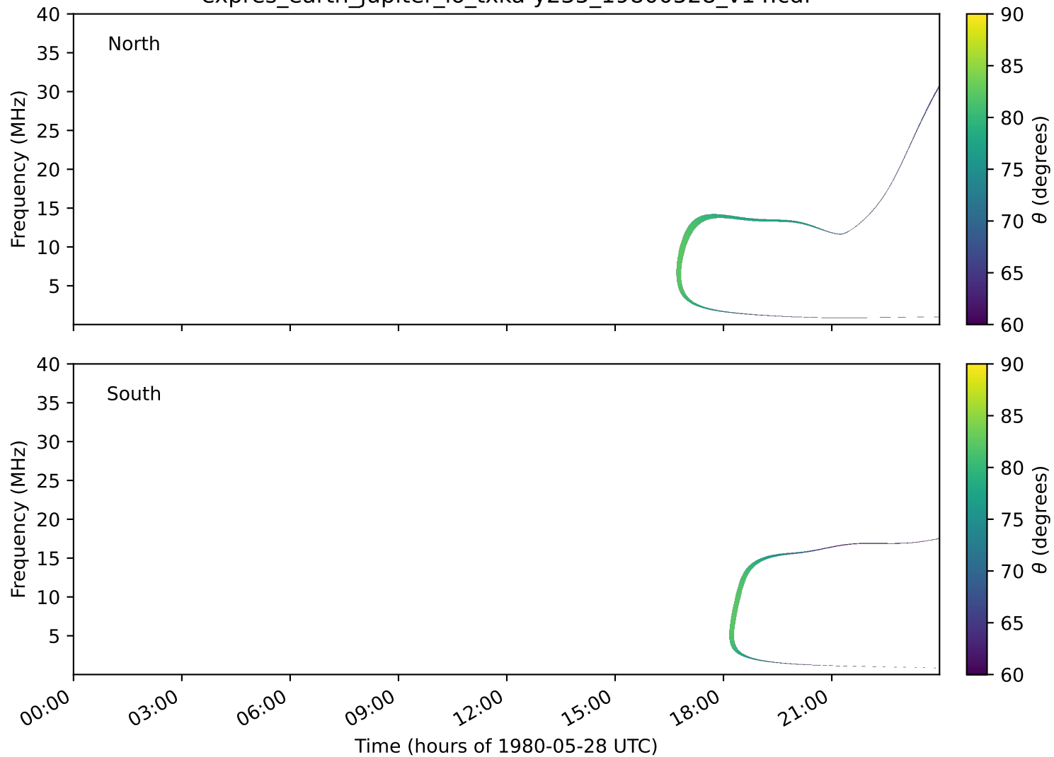
expres_earth_jupiter_io_txka-y235_19800528_v14.cdf
