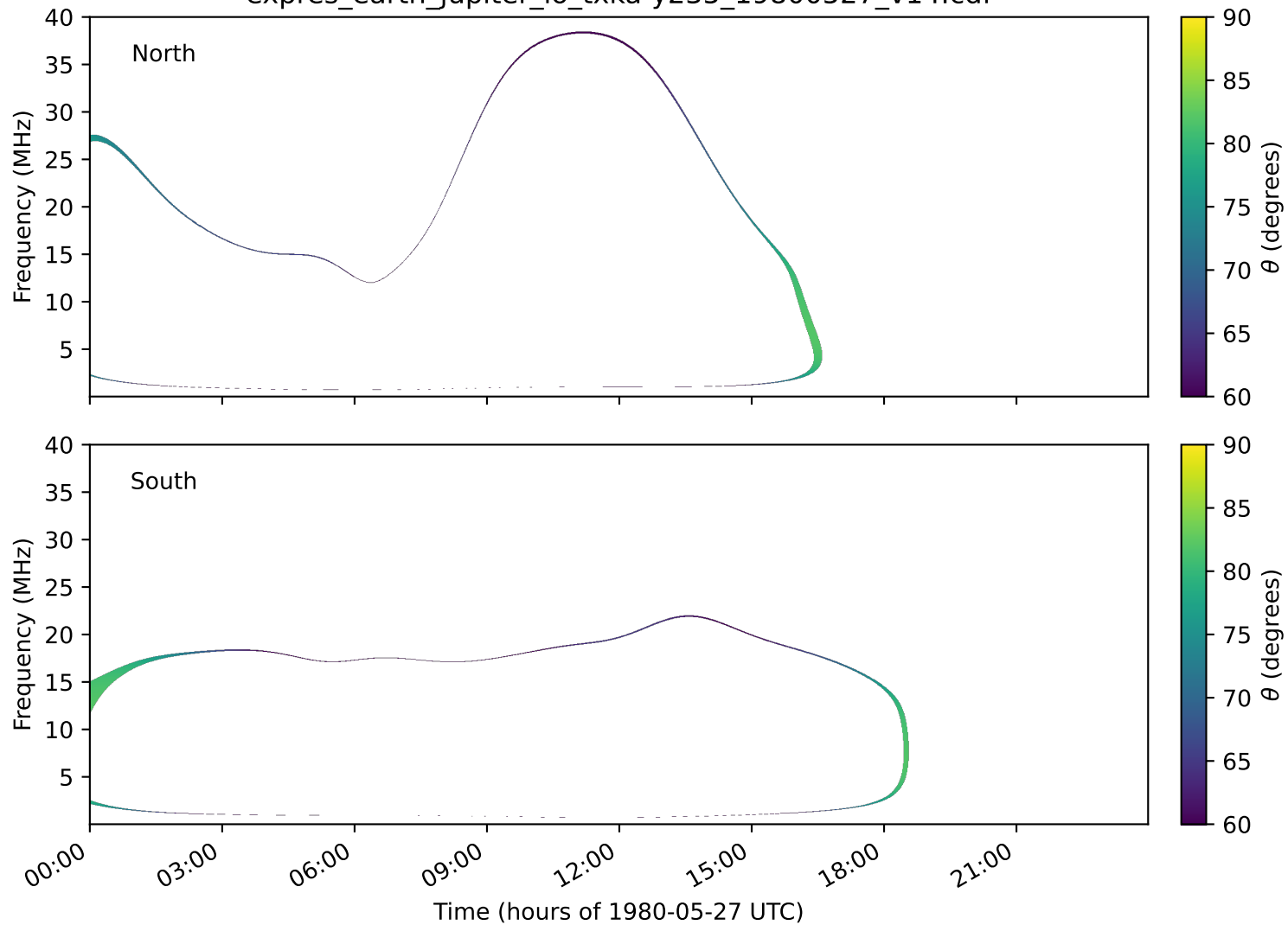
expres_earth_jupiter_io_txka-y235_19800527_v14.cdf
