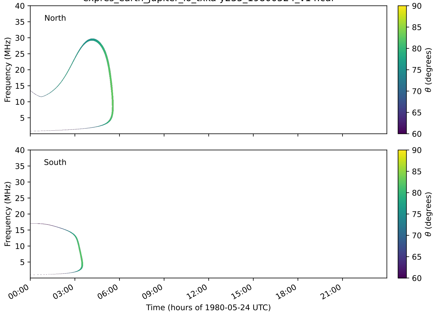
expres_earth_jupiter_io_txka-y235_19800524_v14.cdf
