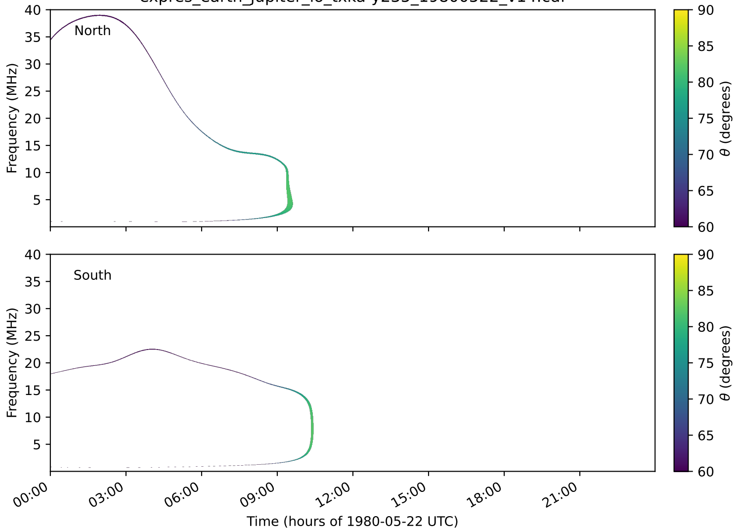
expres_earth_jupiter_io_txka-y235_19800522_v14.cdf
