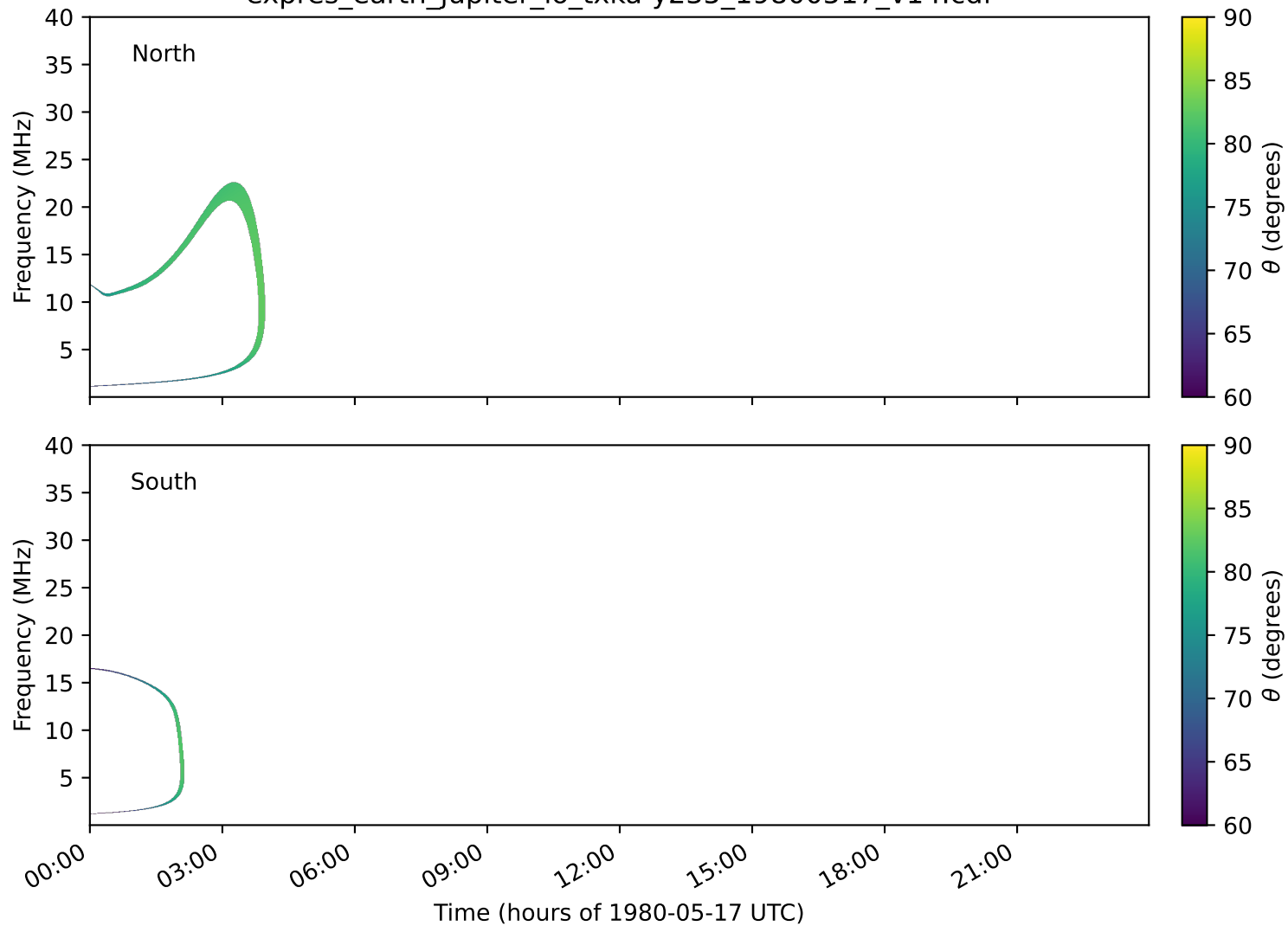
expres_earth_jupiter_io_txka-y235_19800517_v14.cdf
