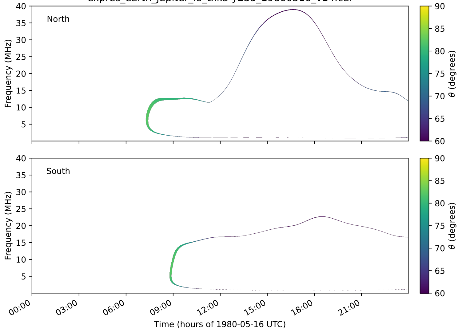
expres_earth_jupiter_io_txka-y235_19800516_v14.cdf
