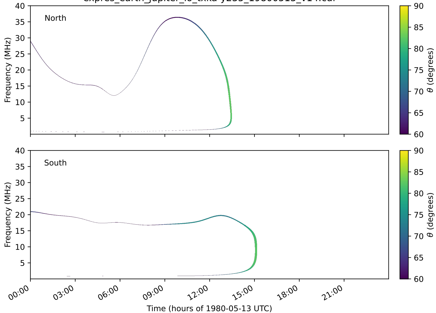
expres_earth_jupiter_io_txka-y235_19800513_v14.cdf
