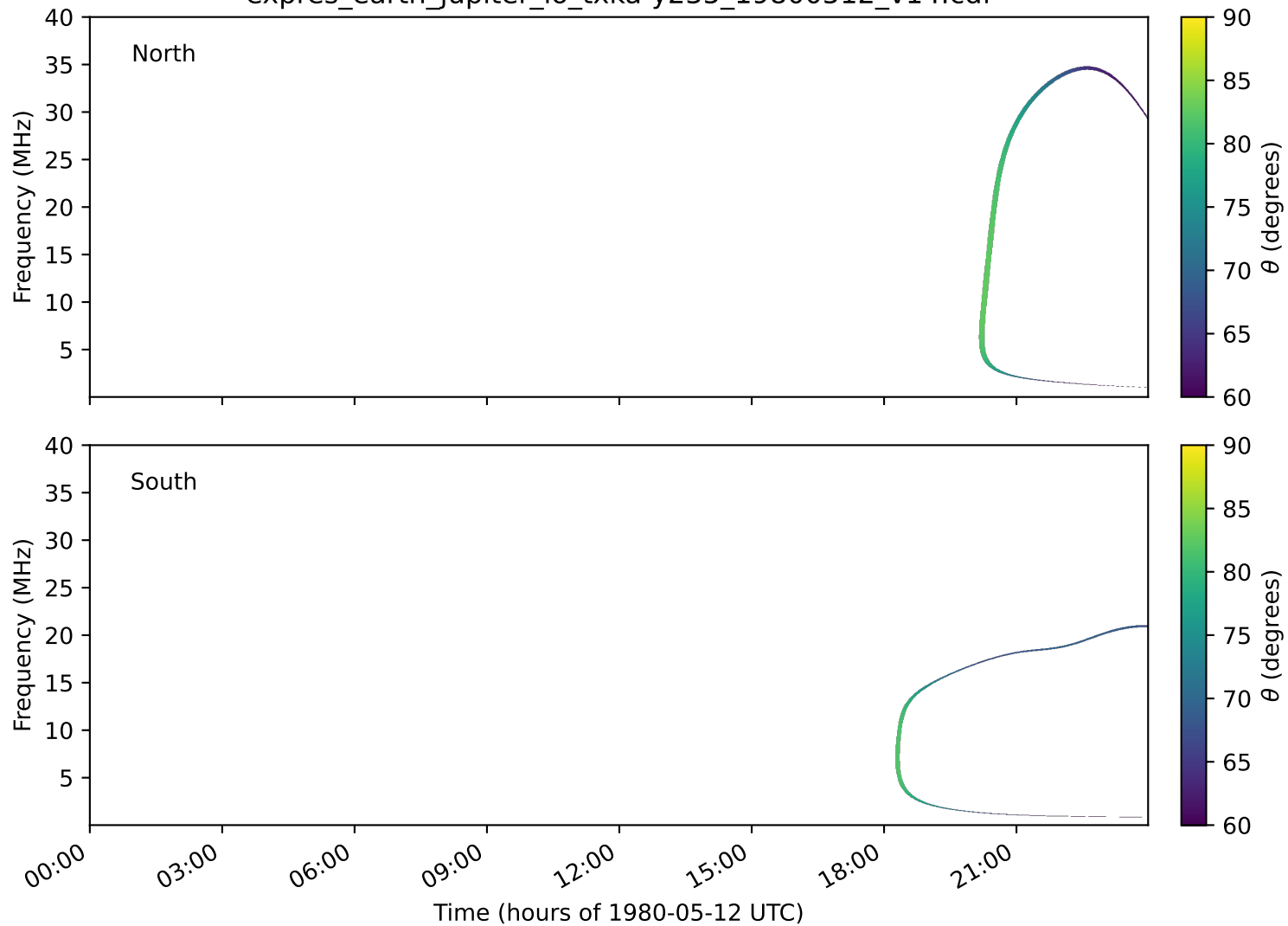
expres_earth_jupiter_io_txka-y235_19800512_v14.cdf
