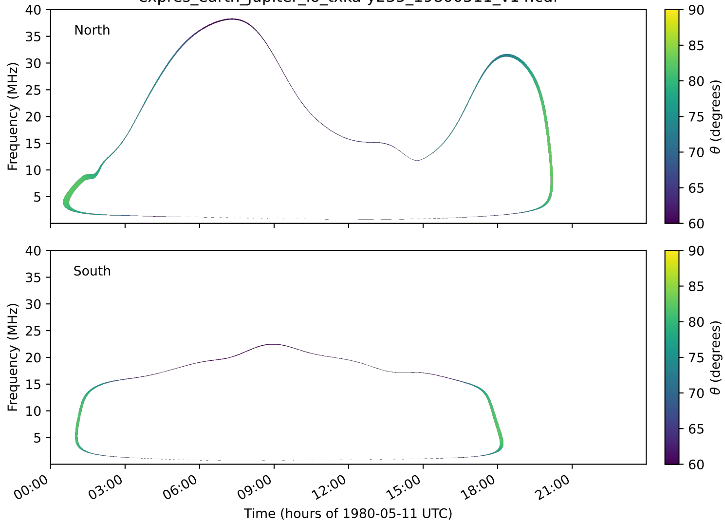
expres_earth_jupiter_io_txka-y235_19800511_v14.cdf
