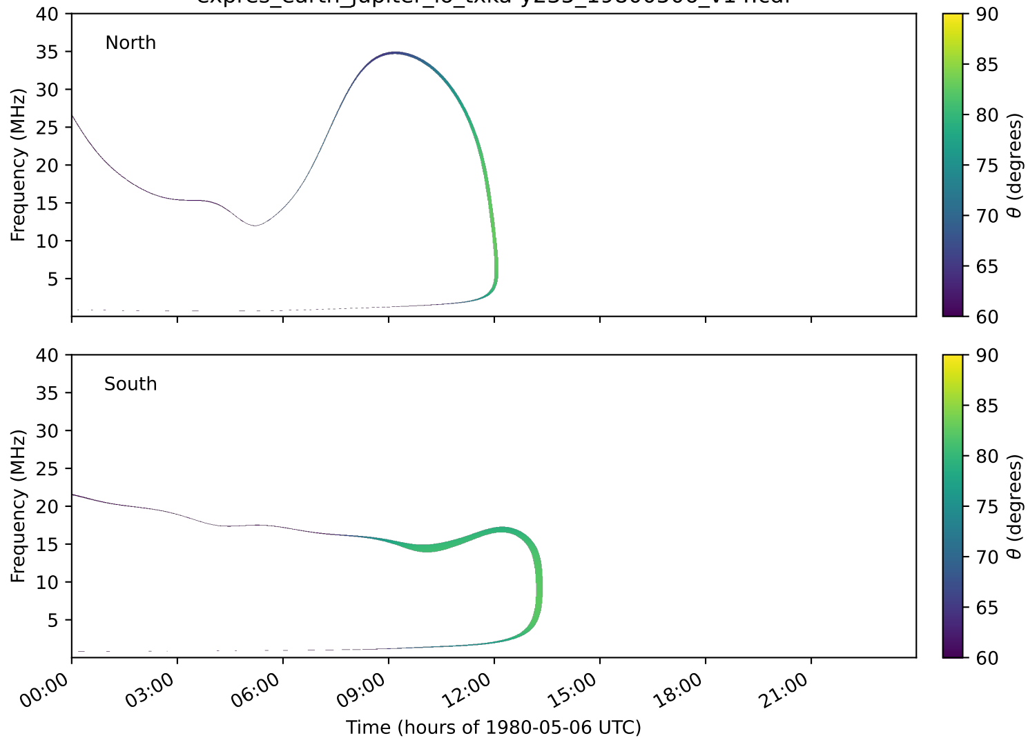
expres_earth_jupiter_io_txka-y235_19800506_v14.cdf
