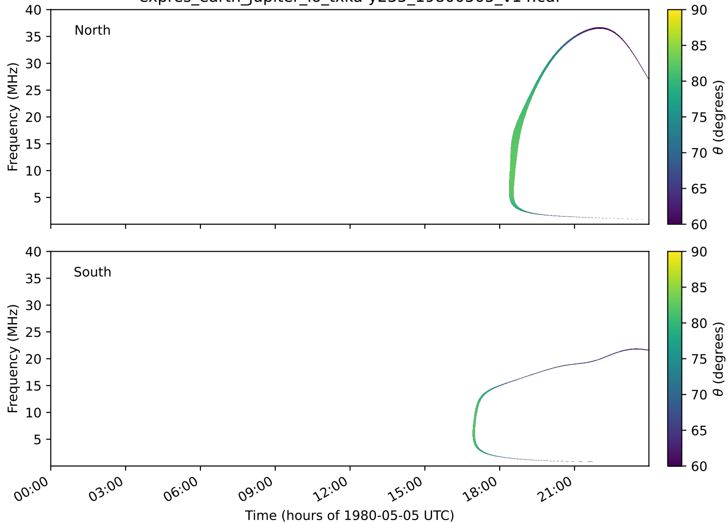
expres_earth_jupiter_io_txka-y235_19800505_v14.cdf
