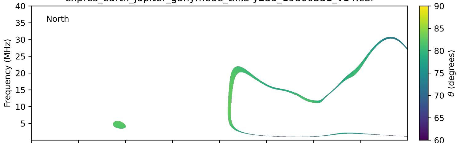
expres_earth_jupiter_ganymede_txka-y235_19800531_v14.cdf
