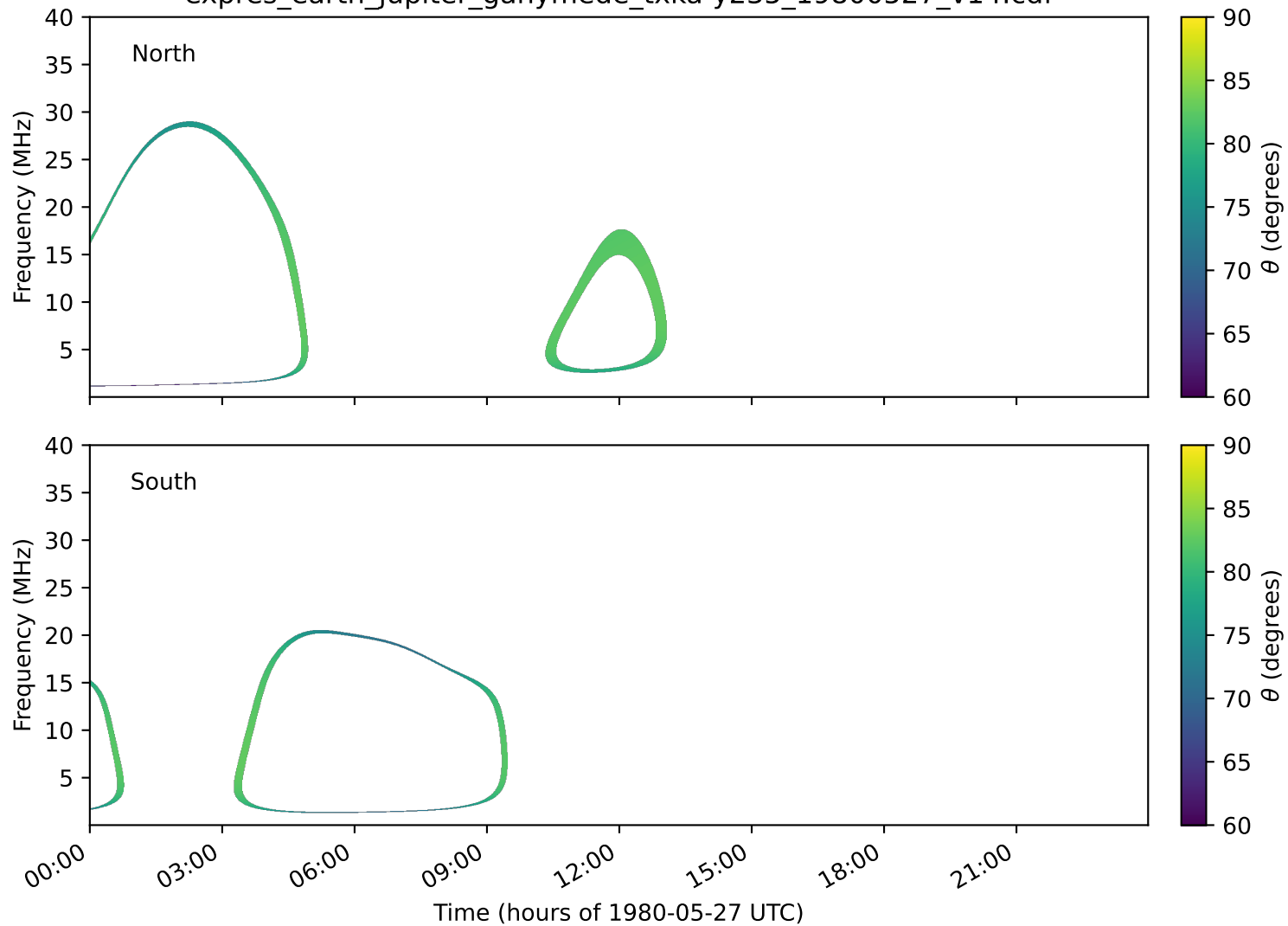
expres_earth_jupiter_ganymede_txka-y235_19800527_v14.cdf
