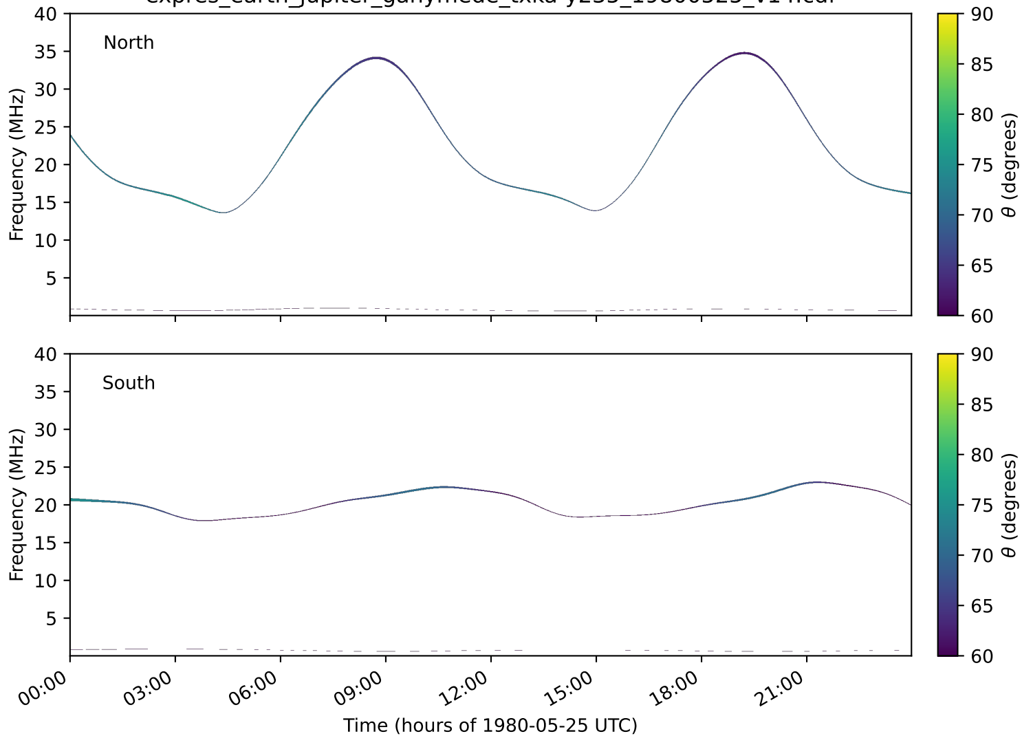
expres_earth_jupiter_ganymede_txka-y235_19800525_v14.cdf
