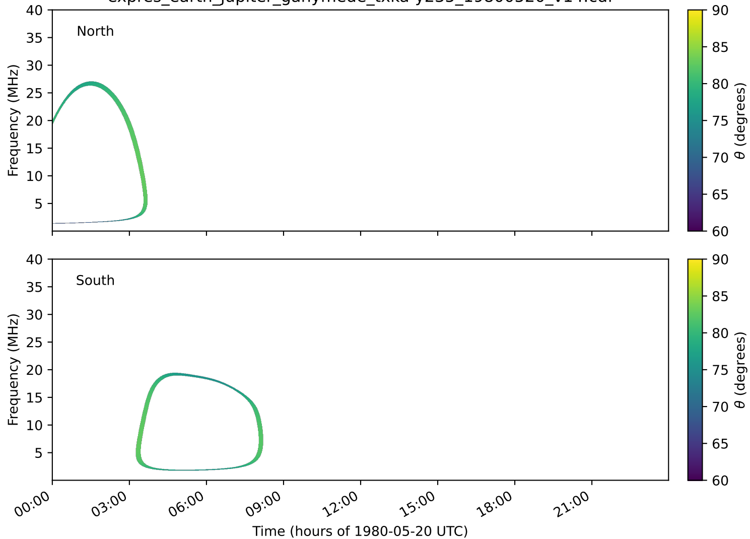
expres_earth_jupiter_ganymede_txka-y235_19800520_v14.cdf
