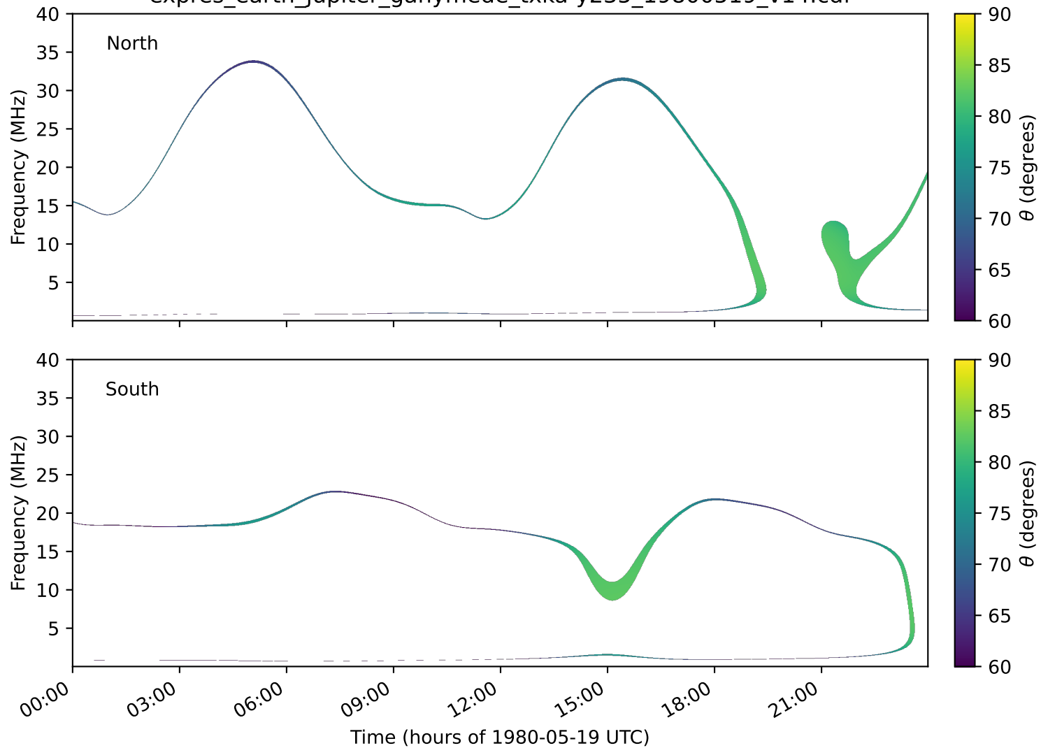
expres_earth_jupiter_ganymede_txka-y235_19800519_v14.cdf
