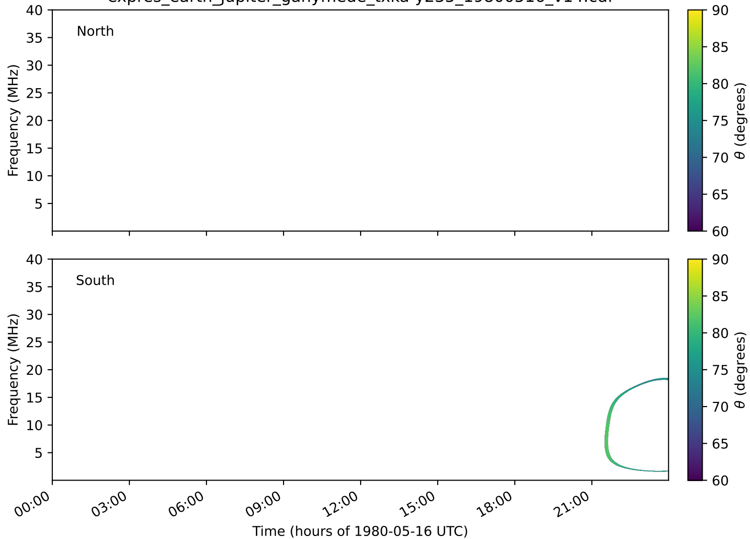
expres_earth_jupiter_ganymede_txka-y235_19800516_v14.cdf
