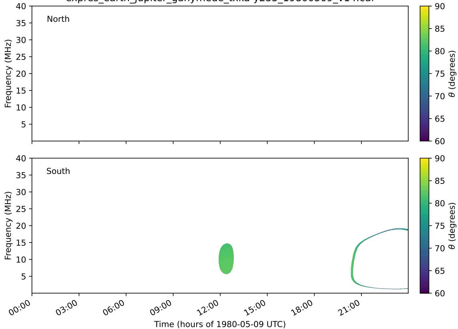
expres_earth_jupiter_ganymede_txka-y235_19800509_v14.cdf
