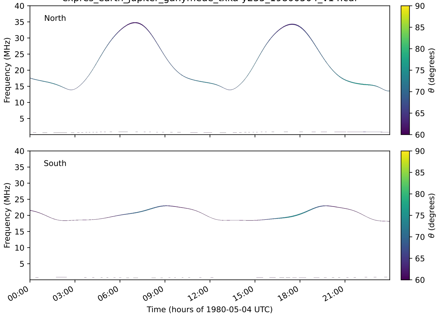
expres_earth_jupiter_ganymede_txka-y235_19800504_v14.cdf
