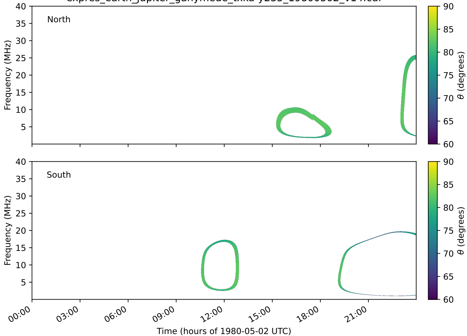
expres_earth_jupiter_ganymede_txka-y235_19800502_v14.cdf
