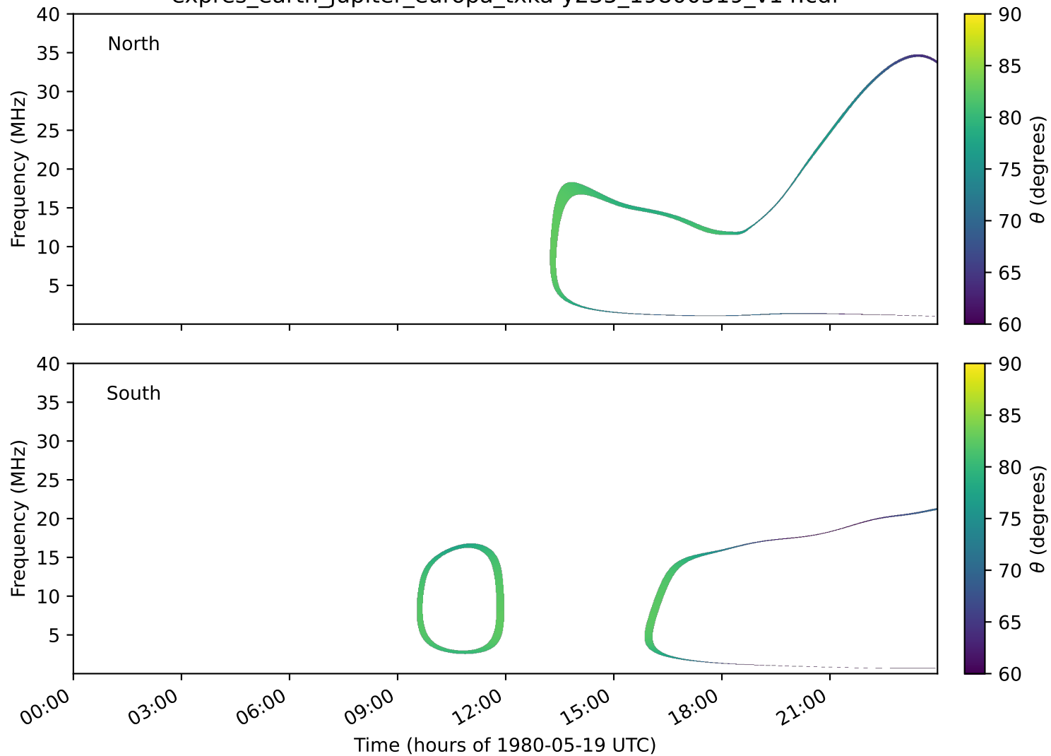
expres_earth_jupiter_europa_txka-y235_19800519_v14.cdf
