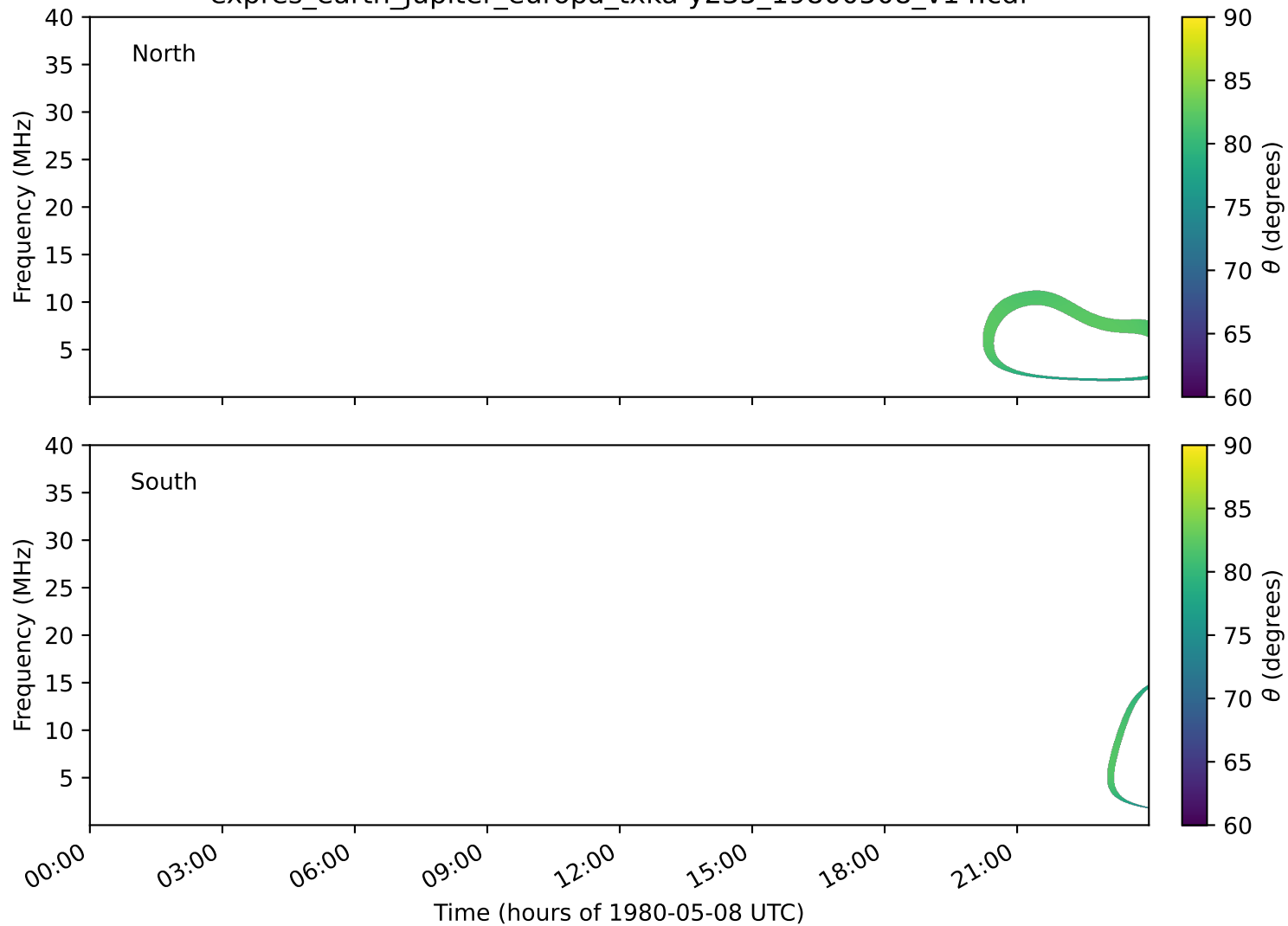
expres_earth_jupiter_europa_txka-y235_19800508_v14.cdf
